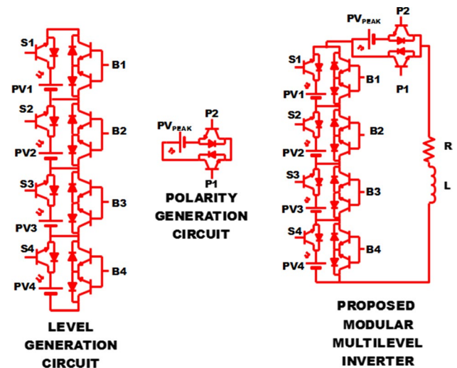
Fig. 2 Proposed MMI
