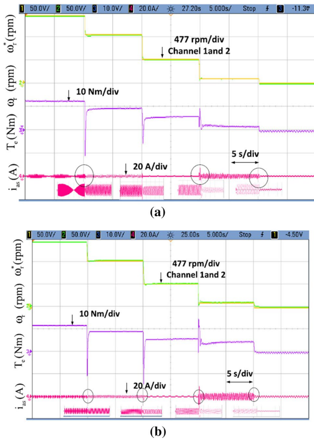
Fig. 23 Transient state performance for case 2 using; a PI controller; b fuzzy controller
