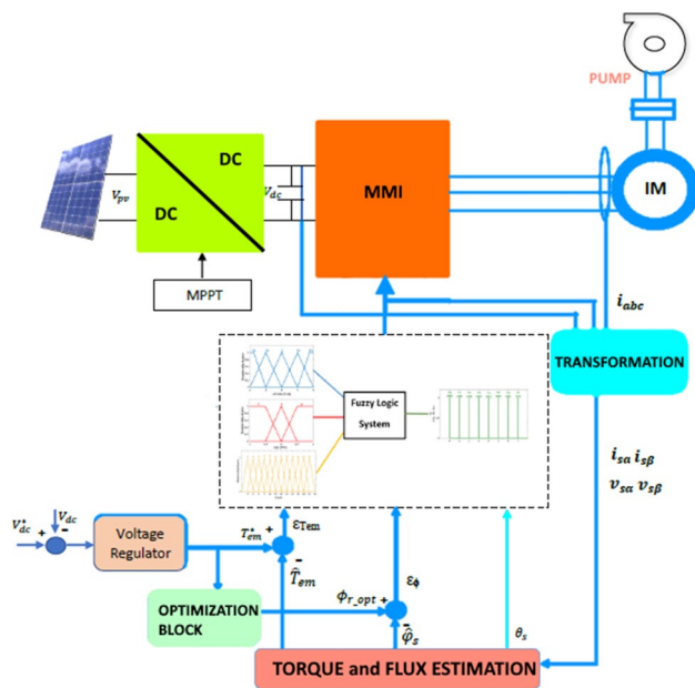
Fig. 9 FLC-based DTC Control of IM
