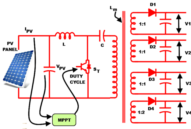
Fig. 5 Simo SEPIC converter
