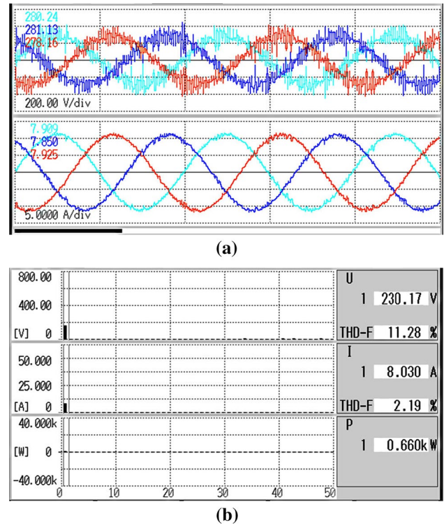
Fig. 24 Experimental output of a stator voltage and stator current; b THD of stator voltage and stator current using PI controller
